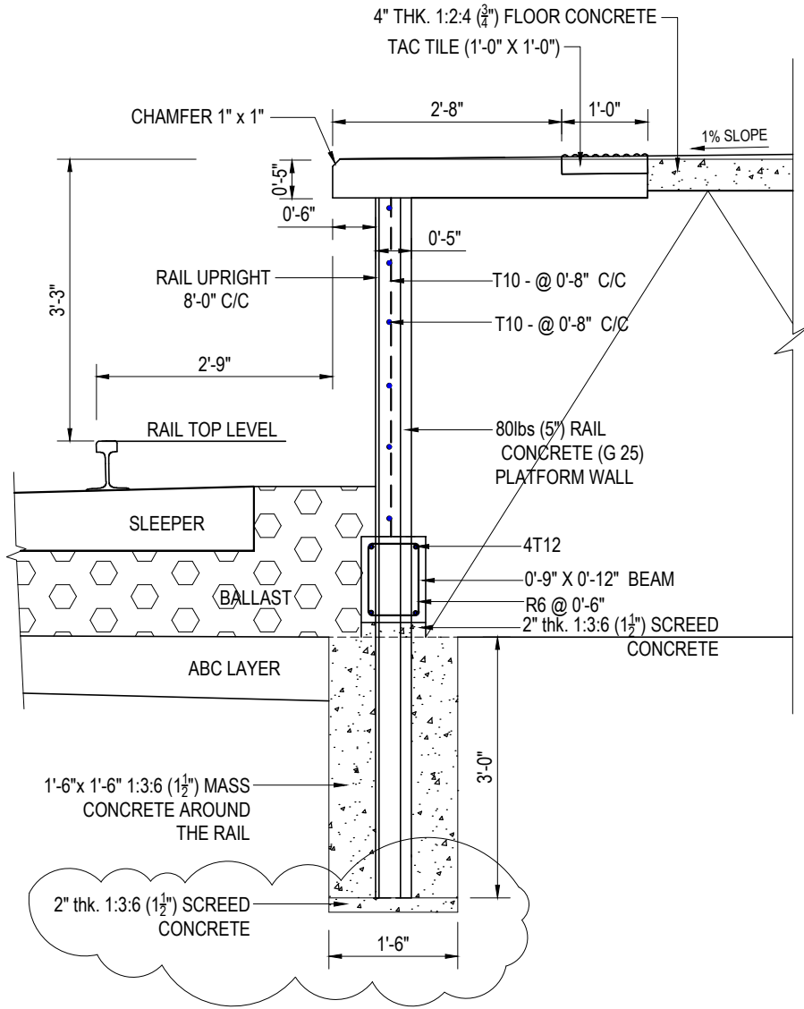
SECTION A-A (SECTION AT RAIL COLUMN) SCALE : 2 FEET TO AN INCH
