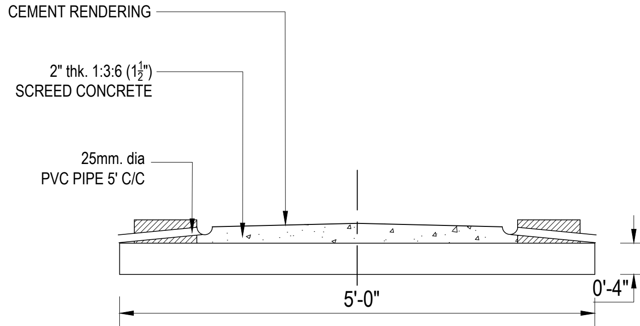
DETAIL OF PRE CAST SLAB PANELS
