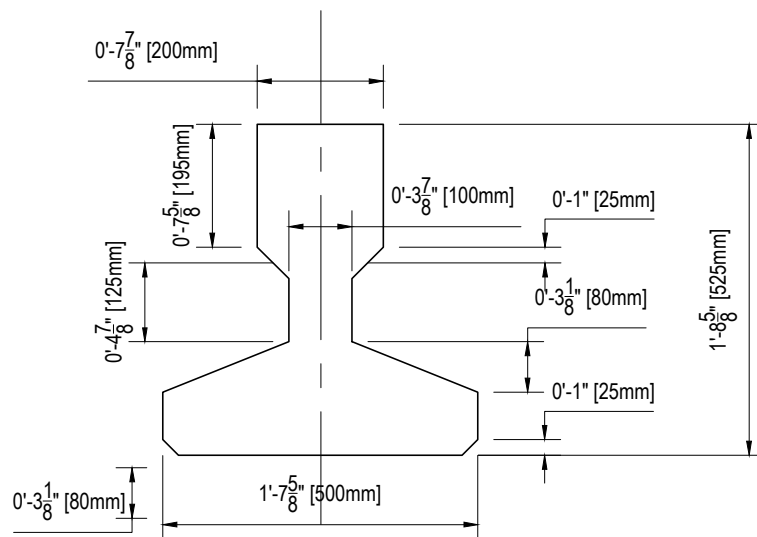
PSC BEAM LENGTH 43'-7" (13.5m)
