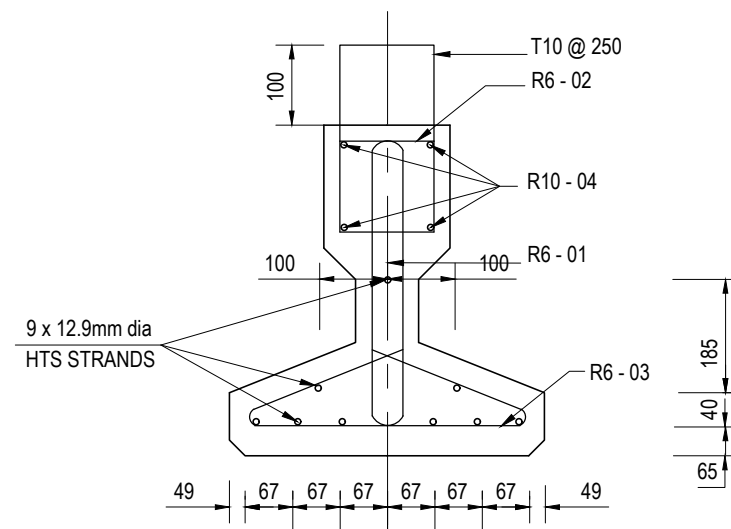
PSC BEAM LENGTH 43'-7" (13.5m)
